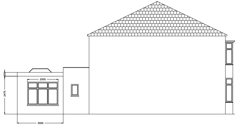
Proposed Left H/S Elevation
