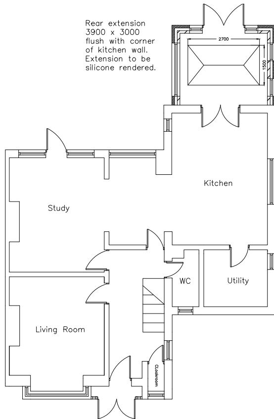
Proposed Ground Floor
